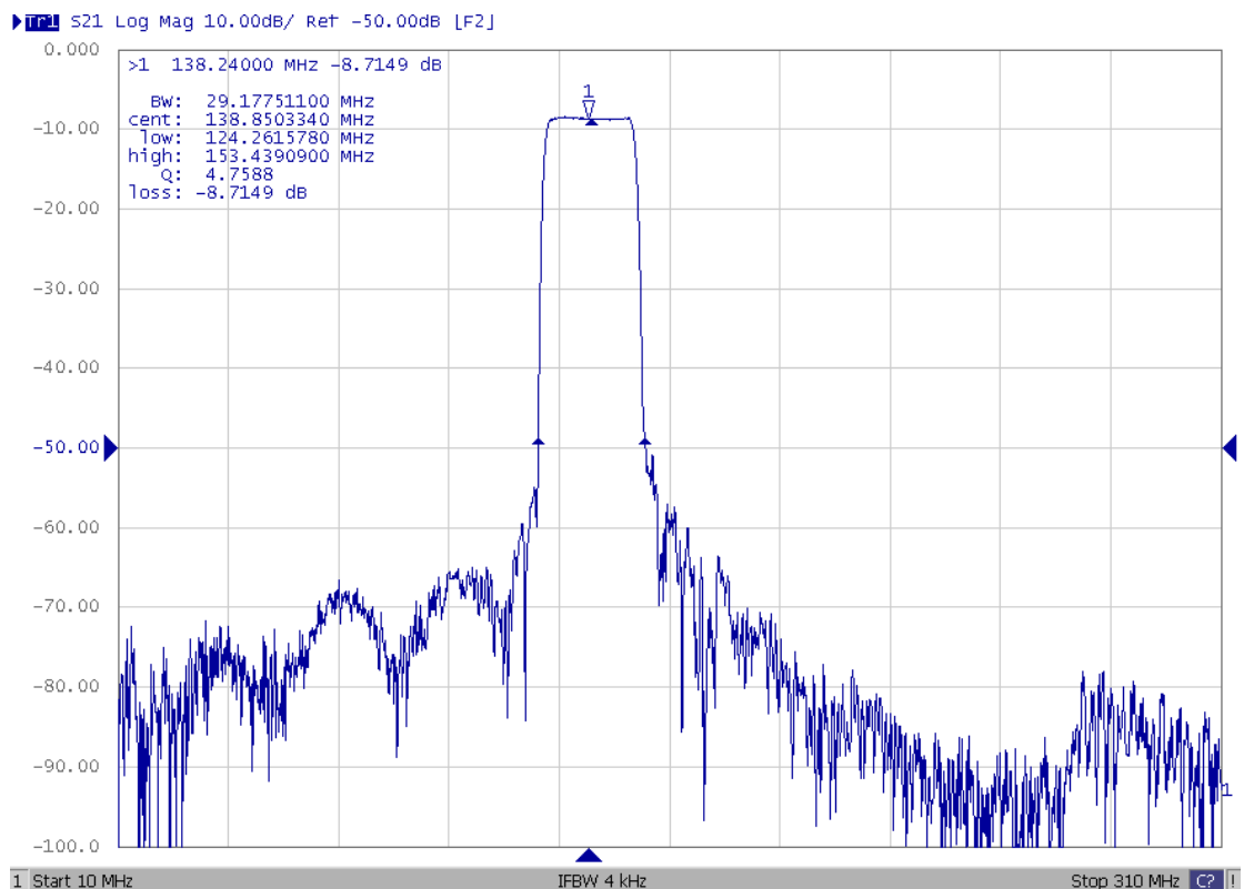
Fig1. Horizontal: 30MHz/Div Vertical: 10dB/Div
